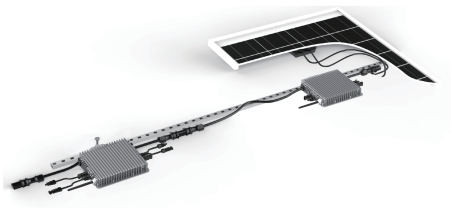
300/500G (1MPPT) 600/800/1000G3 (2MPPT) connect in parallel
