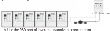
h. Use the RSD port of inverter to supply the concentrator
