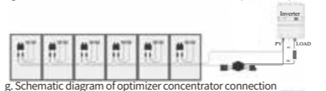
g. Schematic diagram of optimizer concentrator connection
